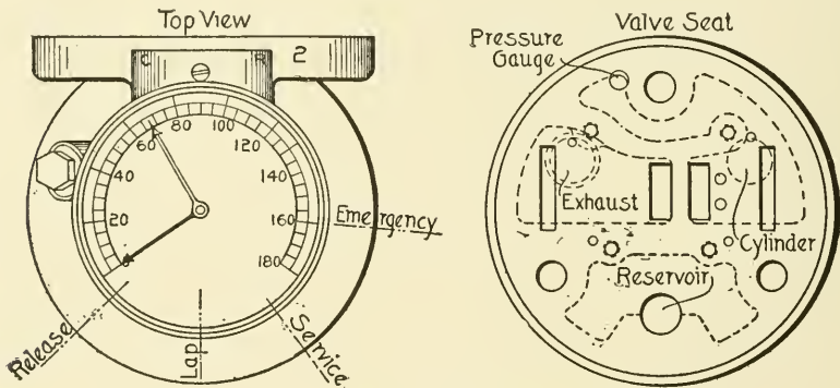
Fig. 95. Top View and Section of Valve Showing Pressure Gauge
